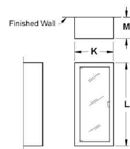
SURFACE
