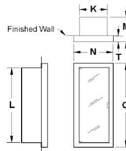
SEMI-RECESSED
