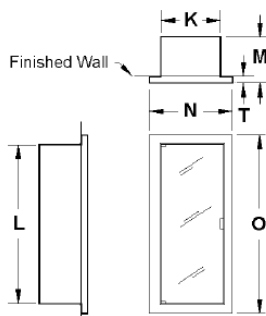
RECESSED
