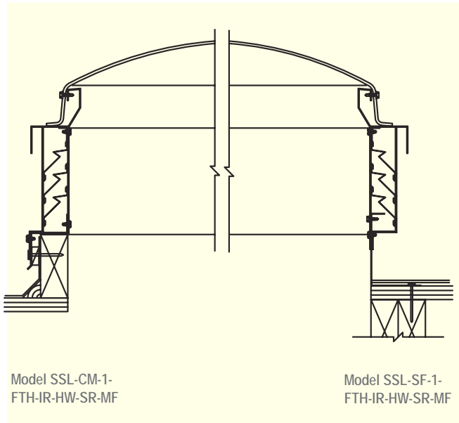
Typical Curb Mount and Self-Flashing Details
