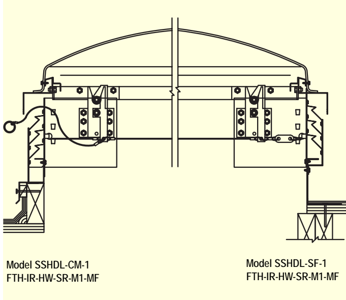
Typical Self-Flashing and Curb Mount Details
