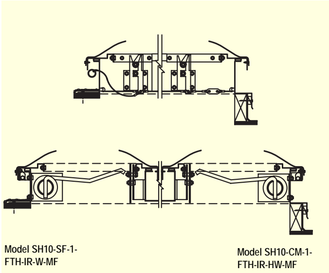
Typical Curb Mount and Self-Flashing Details
