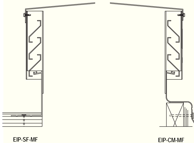
Typical Self-Flashing and Curb Mount Details
